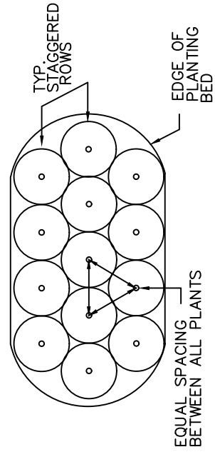
TYPICAL PLANTING BED PLAN
